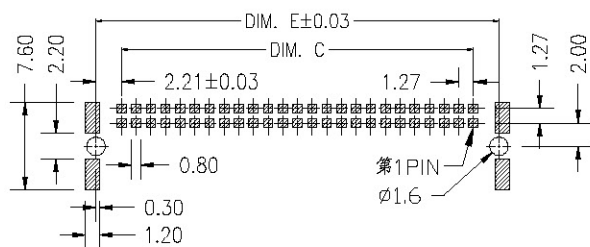
RECOMMENDED PCB LAYOUT (TOLERANCE: ±0.05)
